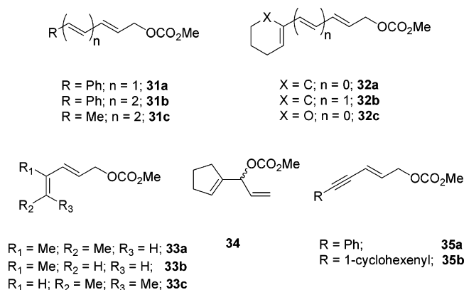
FIGURE 7. Conjugated substrates 31 – 35 .
