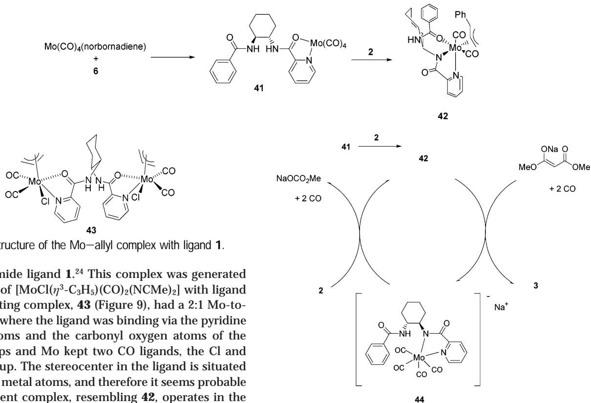
FIGURE 10. Proposed mechanism.
